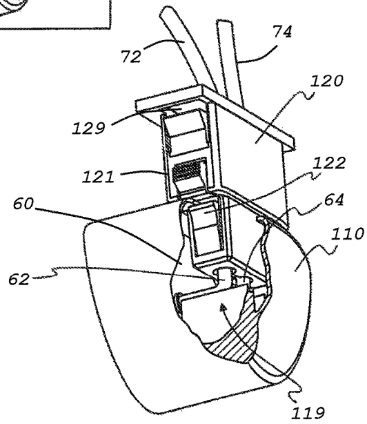
FIG. 7 (Prior Art)
